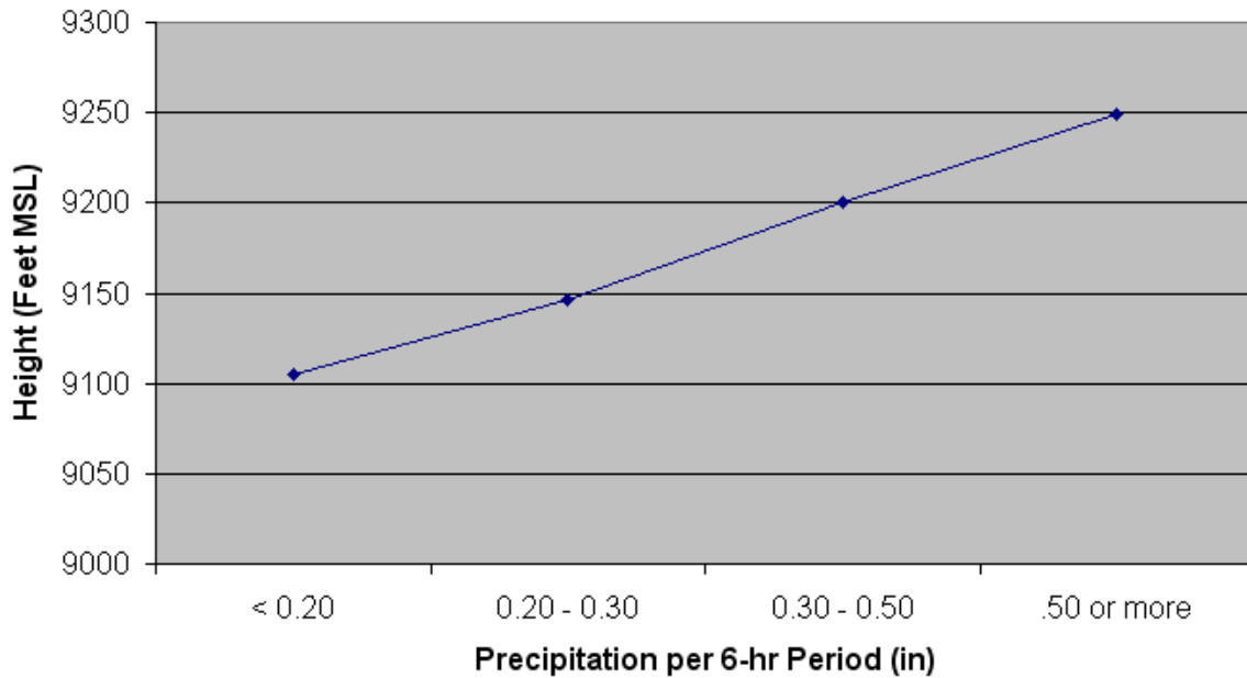
Figure 4.14 Mean Height of the -5^{\circ}\text{C} Isotherm by Precipitation Rate
