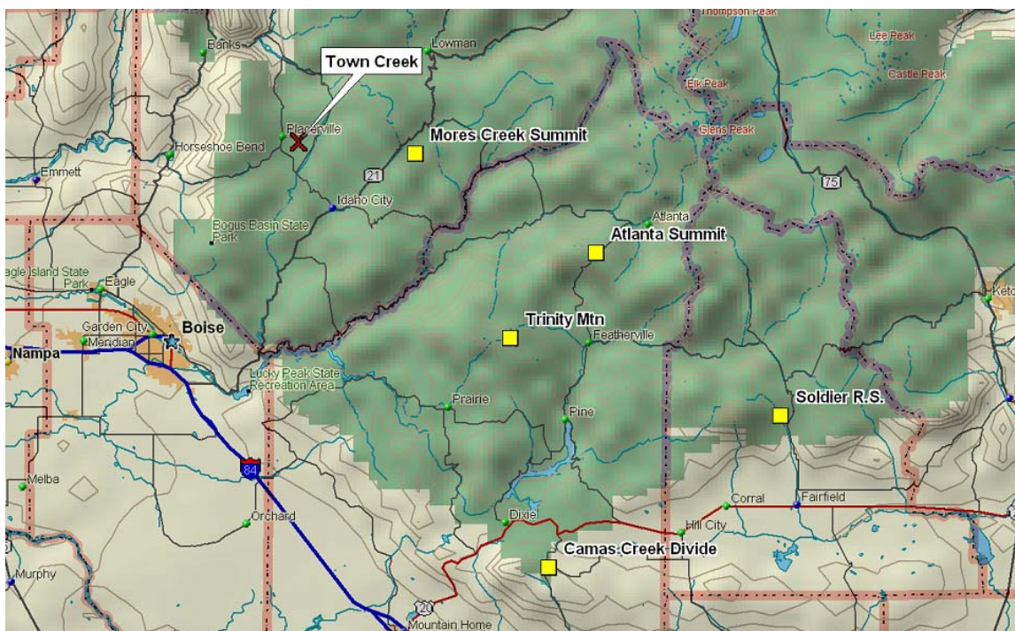
Figure 4.3 Locations of the NRCS Long-term Precipitation and Snowpack Observation Sites
