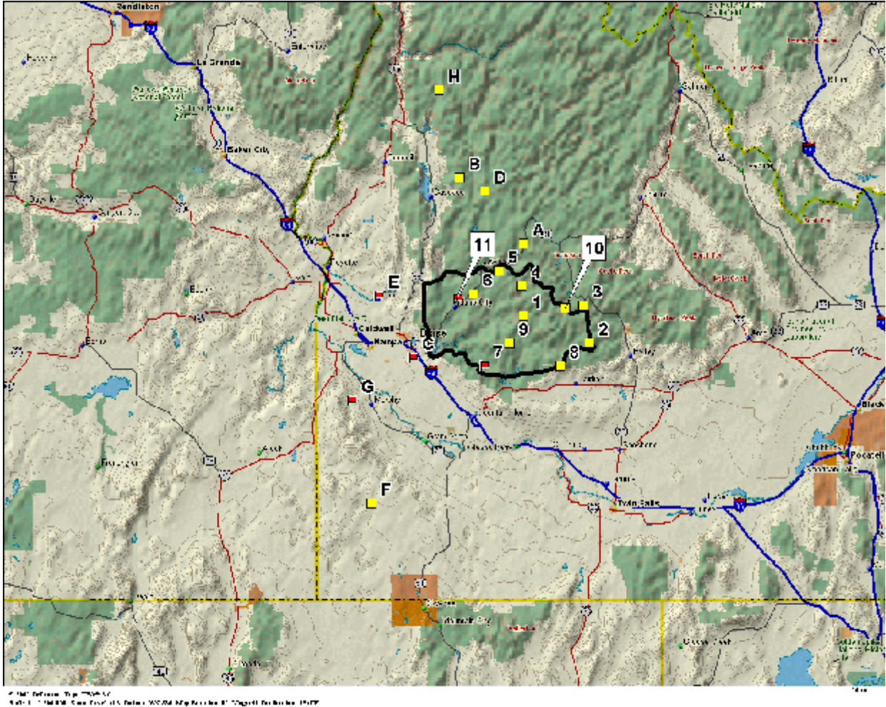
Figure 5.10 Target Sites (numbers) and Original Control Sites (letters) used in earlier Precipitation Evaluations. (Squares represent SNOTEL sites, and flags are NWS cooperative stations; labels correspond to Tables 5-7 and 5-8)
