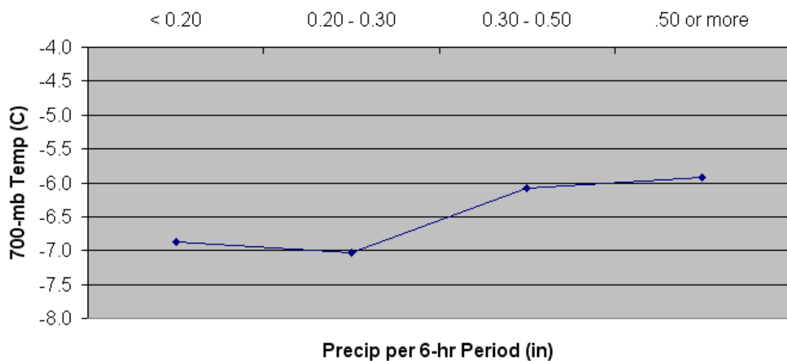
Figure 4.13 Mean 700-mb Temperature by Precipitation Rate
