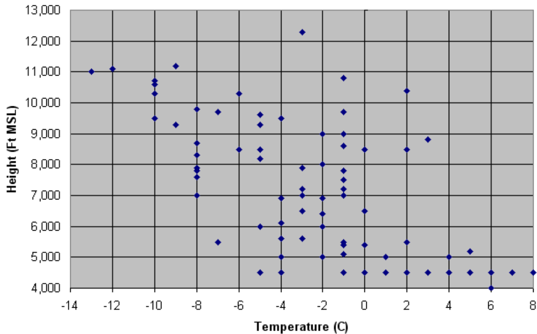
Figure 7.4 Cloud Base Height and Temperature Estimates for all Seedable Periods
