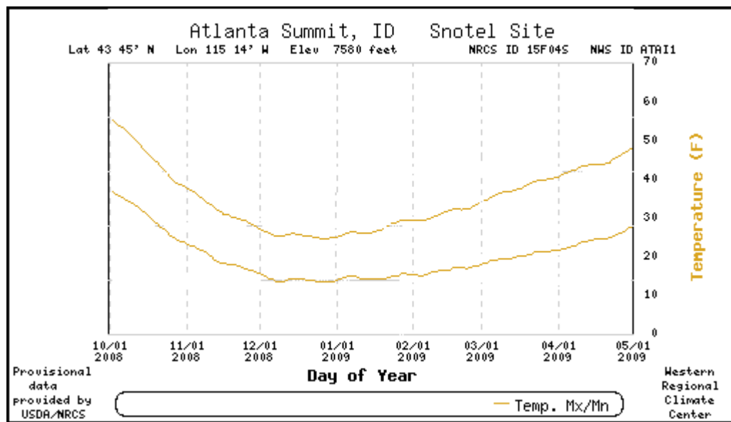
Figure 4.6 Average Winter Season Max/Min Temperature ( ^{\circ} F) at Atlanta Summit SNOTEL Site
