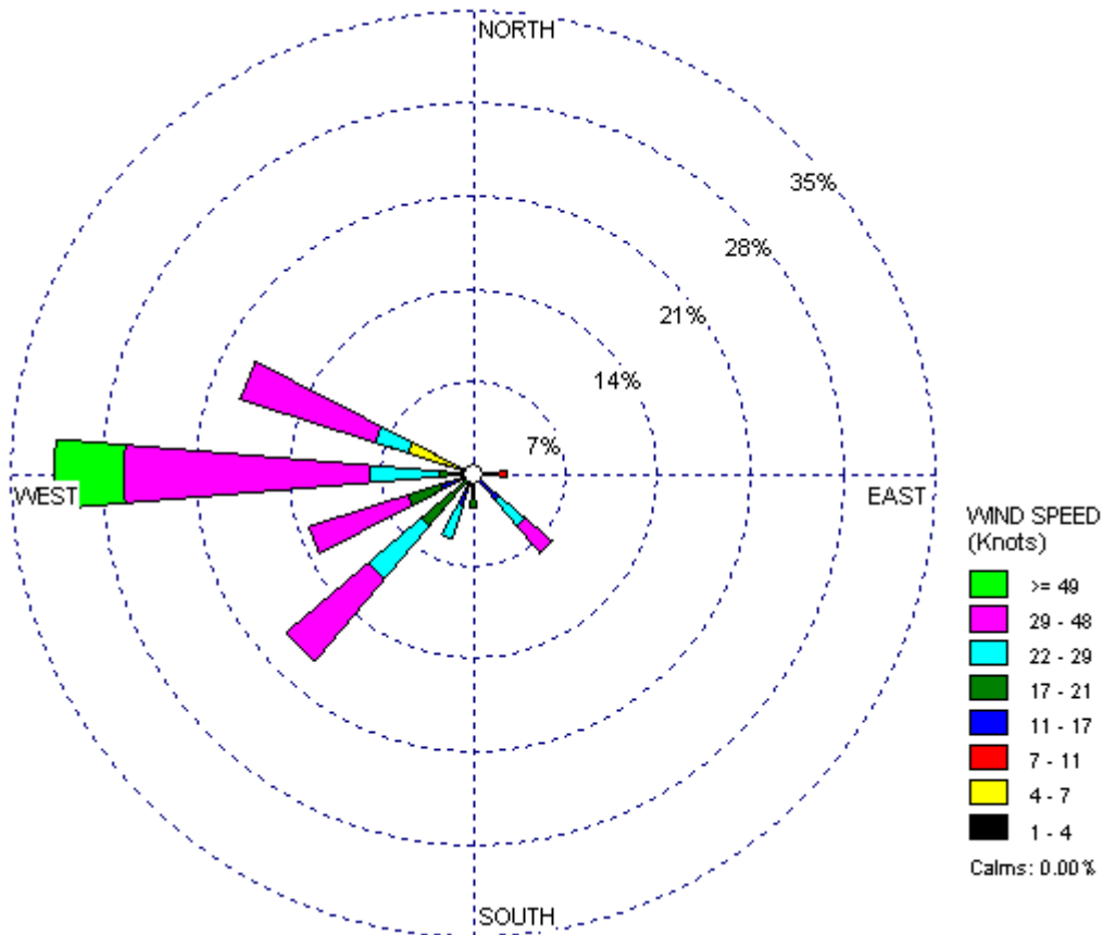
Figure 4.11 700-mb Wind Rose for Aircraft-only Seedable Events
